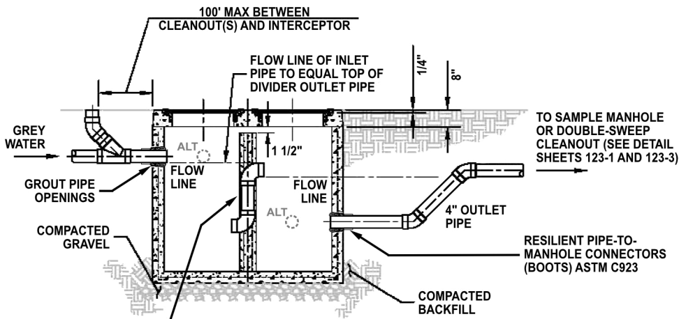
SECTION A
